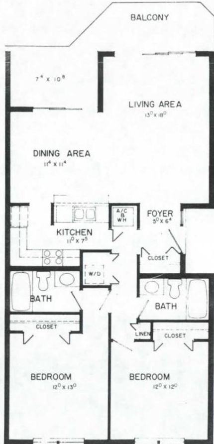
APARTMENT 4 – BUILDINGS C, E, F, H, J, L, N, Q, R – AS SHOWN APARTMENT 3 – BUILDINGS B, D, E, G, H, K, M, P, Q – REVERSE
