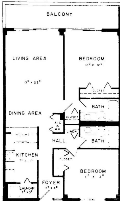
APARTMENT 703 AS SHOWN 709 - REVERSE
