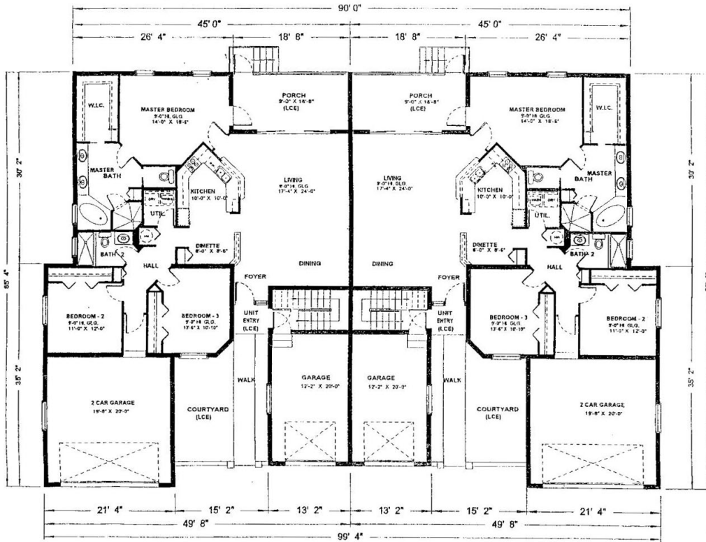
Waterway Cove First Floor Plan www.buymarco.com
