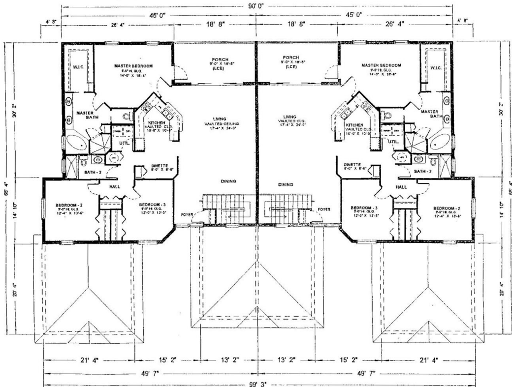
Waterway Cove Second Floor Plan www.buymarco.com
