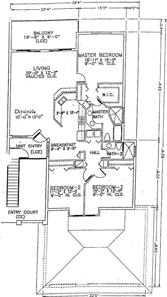
Waterway Pointe Unit 202 - B Floor Plan www.buymarco.com
