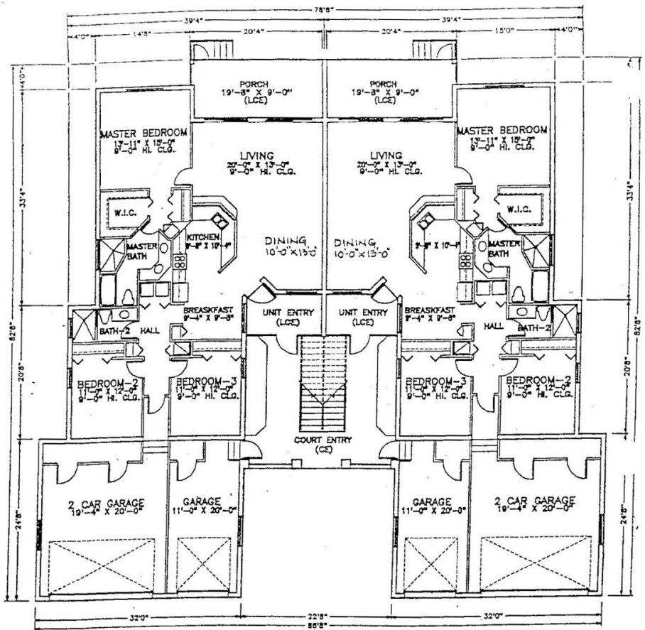
Waterway Pointe First Floor Plan www.buymarco.com
