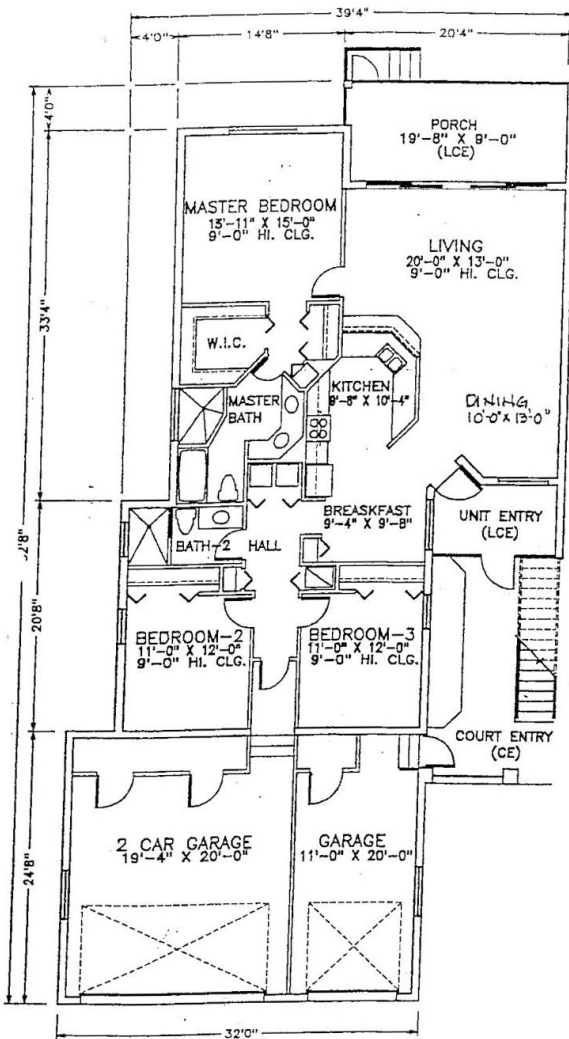
Waterway Pointe Unit 101 - A Floor Plan www.buymarco.com
