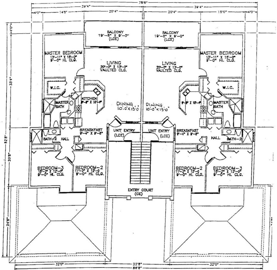
Waterway Pointe Second Floor Plan www.buymarco.com
