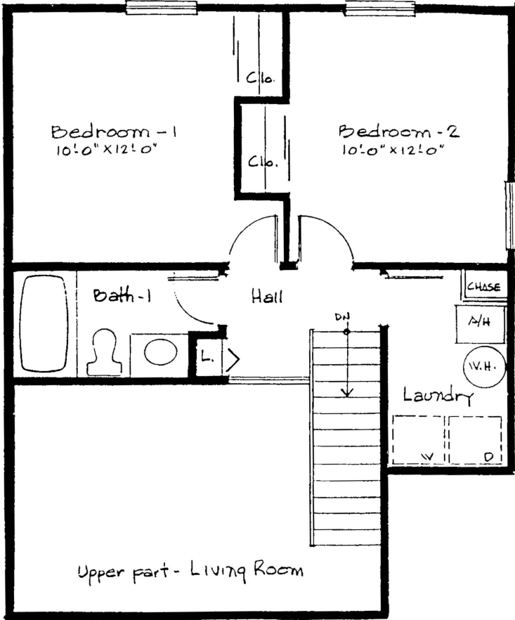
Island Village Second Floor Unit Plan www.buymarco.com
