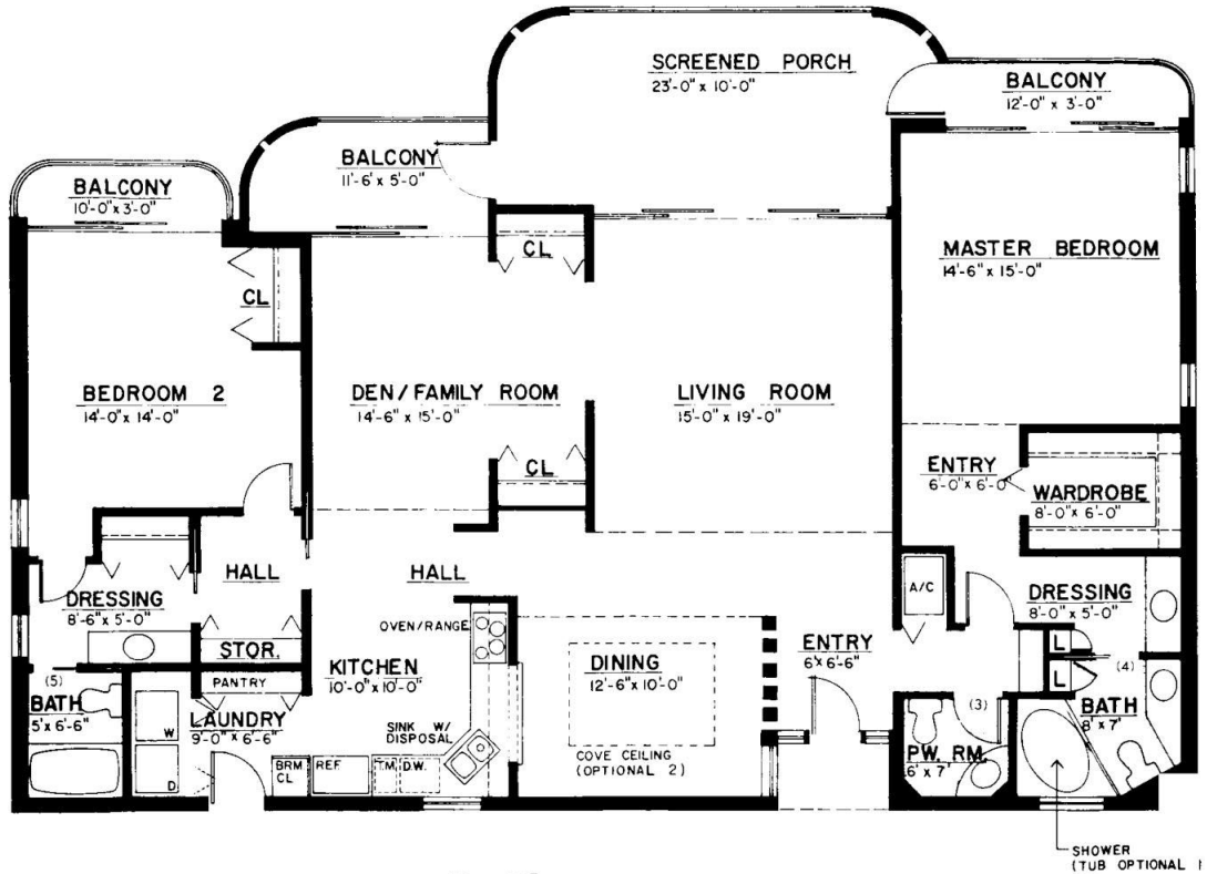
Nautilus Typical Apartment A Total Area 2.210 Sq. Ft. www.buymarco.com
