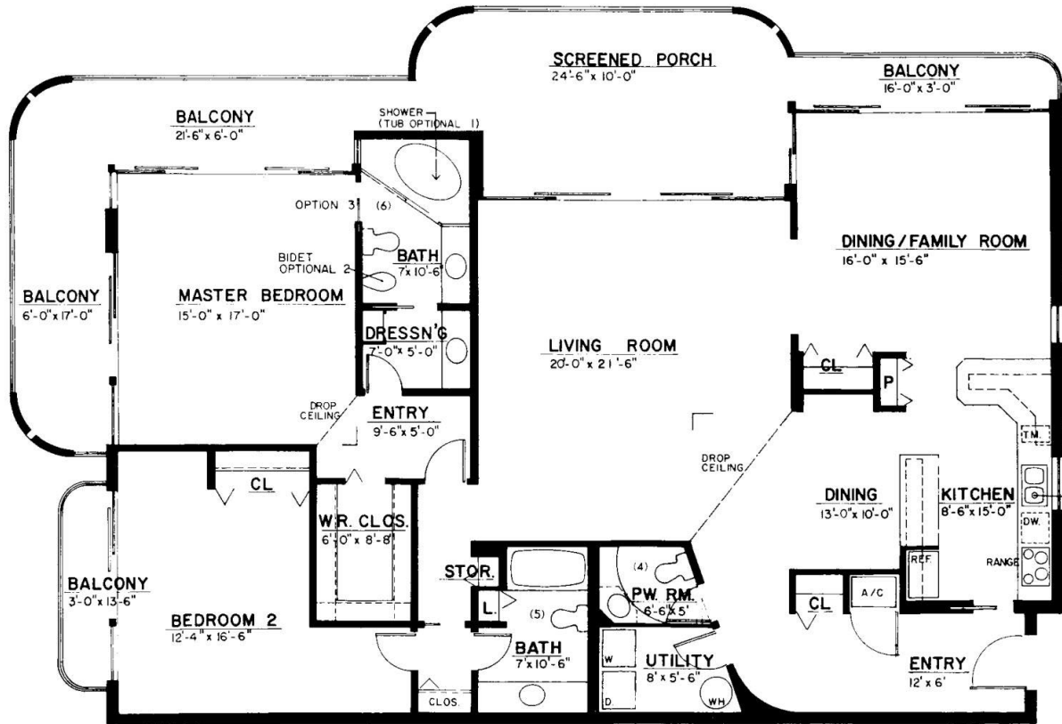
Nautilus Typical Apartment B Total Area 2.680 Sq. Ft. www.buymarco.com
