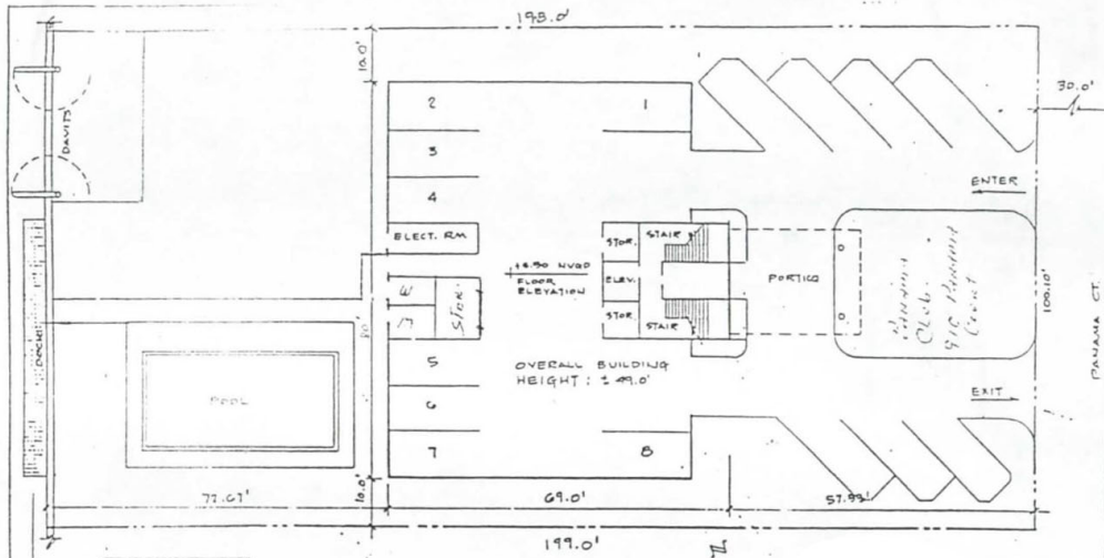
199.0' PLOT PLAN 1" = 20'-0"
